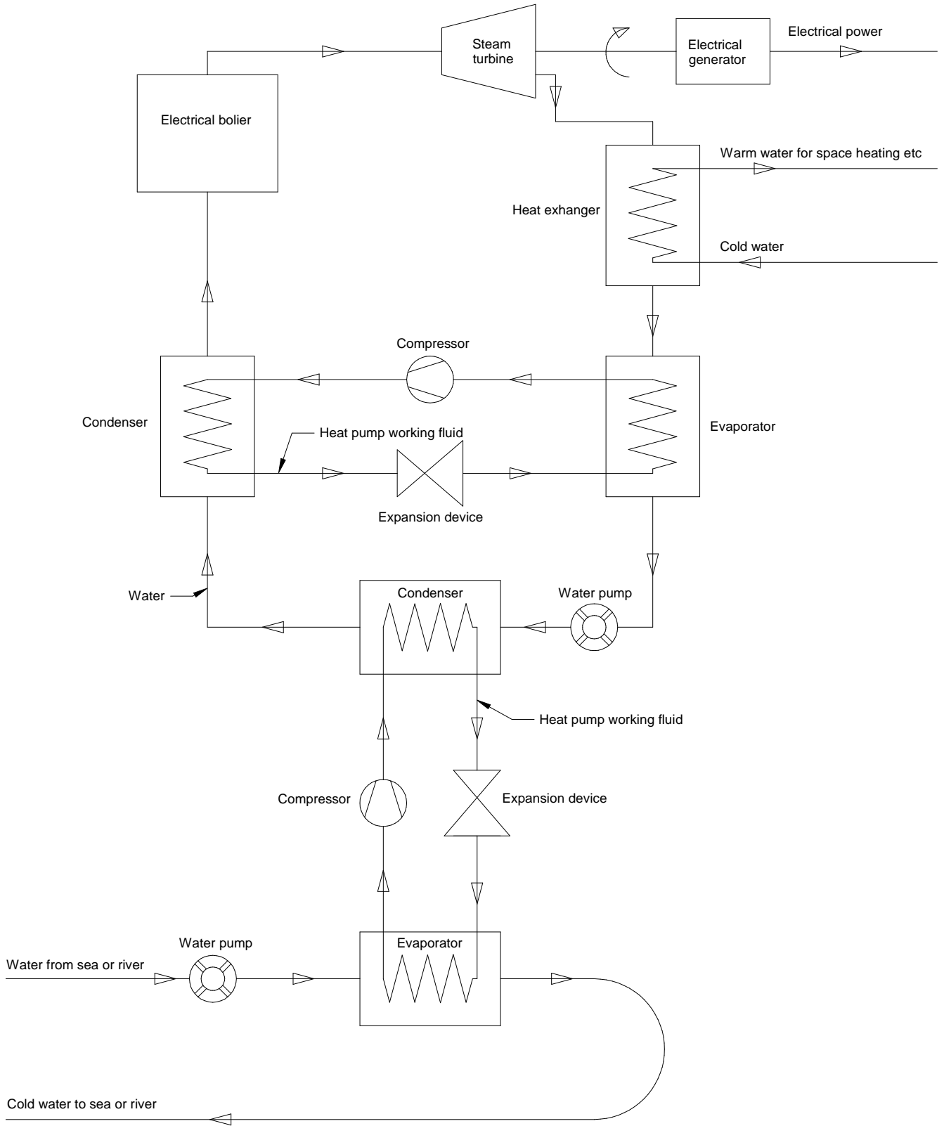
Figure 1 - Schematic of a thermal energy power plant
